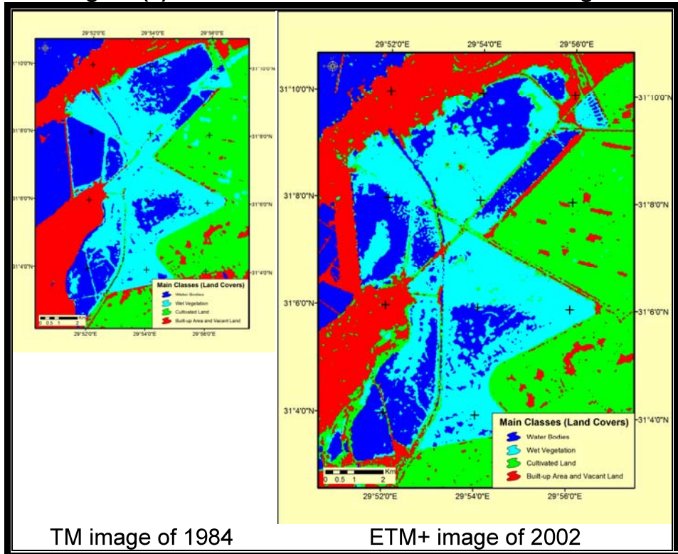
Figure (4): Landsat TM and ETM+ classified images
