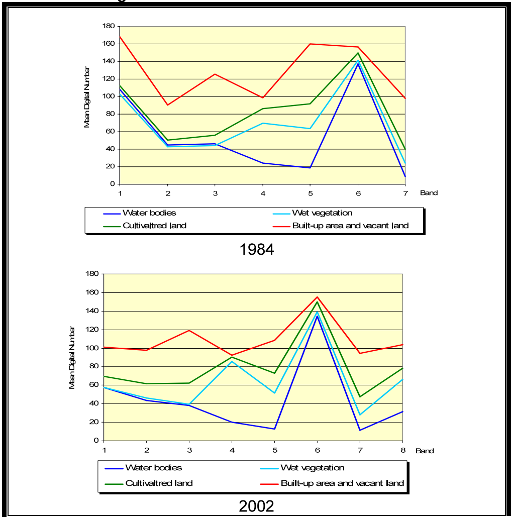
Figure (3): Multiple plots of the spectral signatures of the generated classes in different bands
