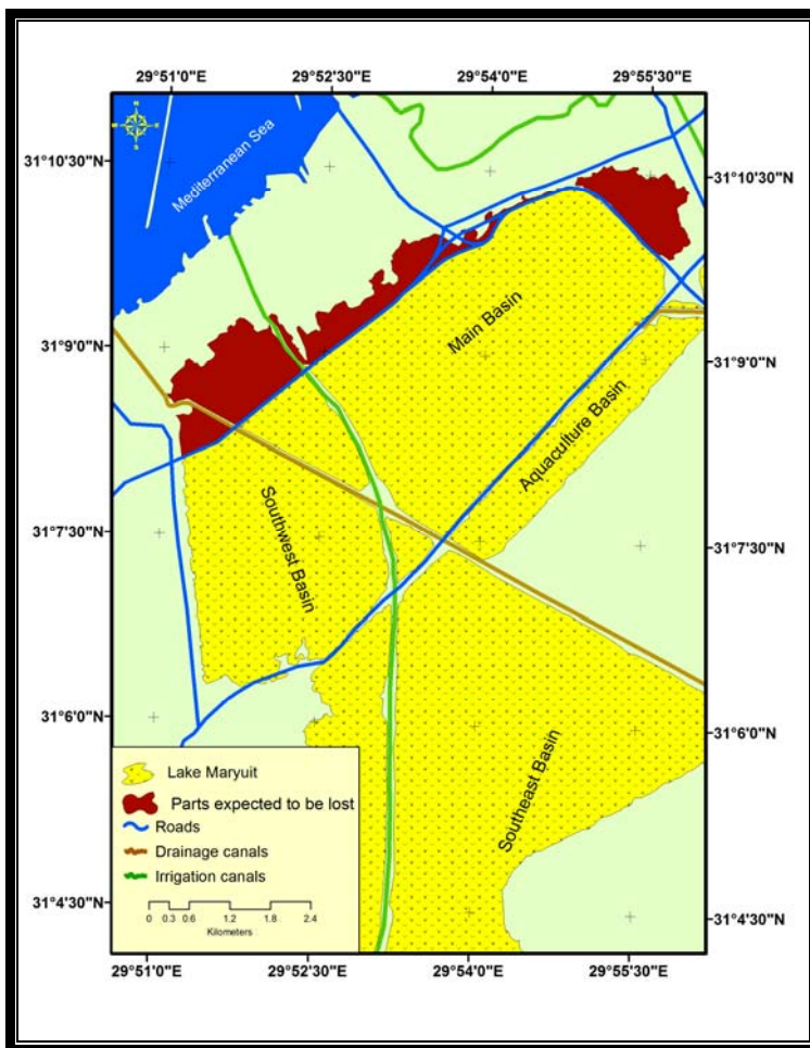
Figure (6): Areas of the lake with higher probability of being land filled in the near future
