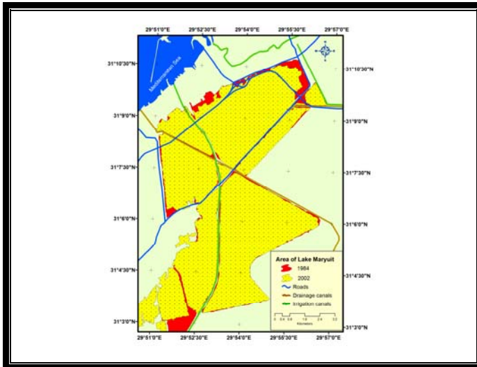
Figure (5): Changes of Lake Maryuit area between 1984 and 2002
