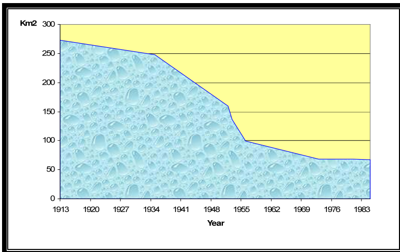
Figure (2): Change of Lake Maryuit Area During 20 th Century
