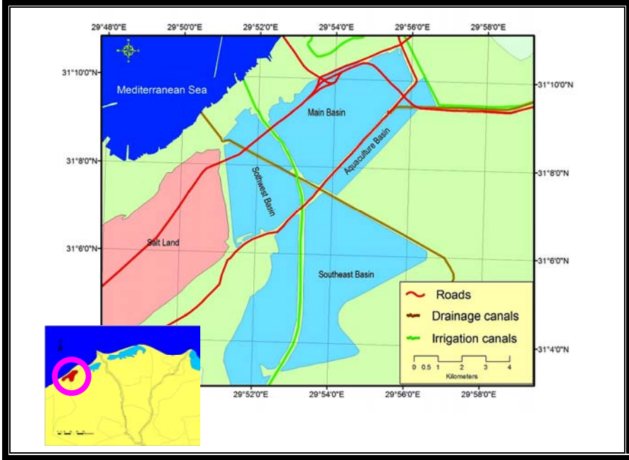
Figure (1): Main basins of Lake Maryuit
