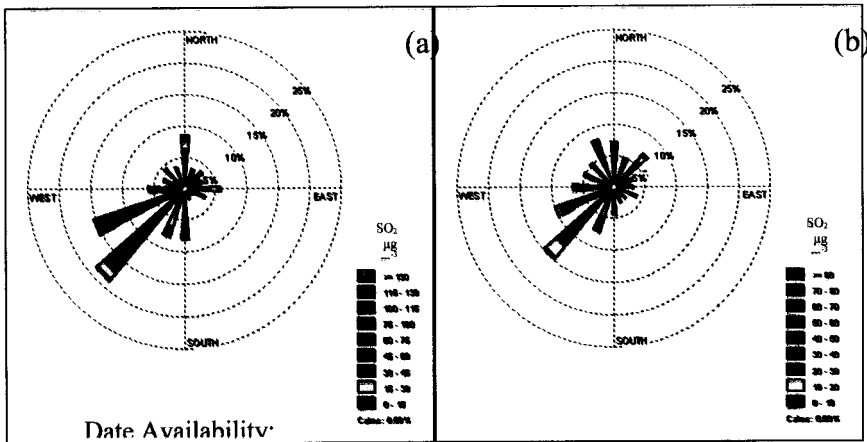
Figure (3). Hourly SO 2 pollution roses for Langdon Cliff station (by using the wind directions for Langdon Cliff), 2001 (a) and 2002 (b).
