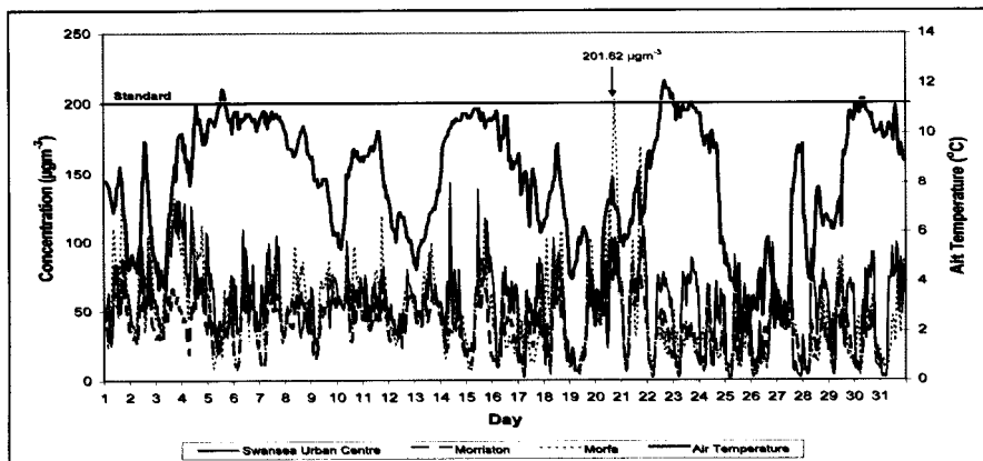
Figure 4). (a) Comparison for the Swansea Urban Centre, Morrision and Morfa station between NO 2 and air temperature, December 2004. Air temperature data from Mumbles Head station and (b) Hourly NO 2 pollution rose for Morfa station (by using the direction for Mumbles Head station), 20th December 2004.
